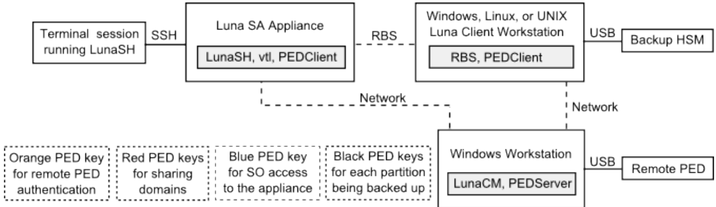
Figure 4: Configuration for remote backup of a Luna SA appliance with the remote PED connected to a separate workstation
